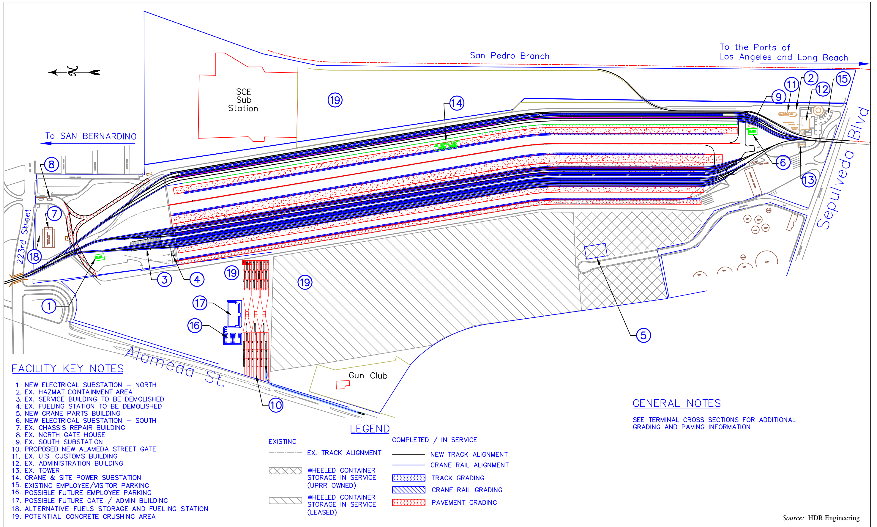
Figure 5. Proposed ICTF Modernization Project Site Plan
